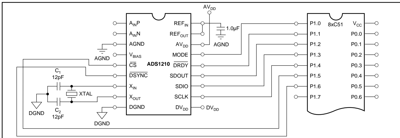
FIGURE 31. Full Interface With a 8xC51 Processor.
