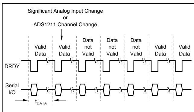
FIGURE 4. ADS1210/11 Analog Input Voltage Step or ADS1211 Channel Change to Fully Settled Output Data.
