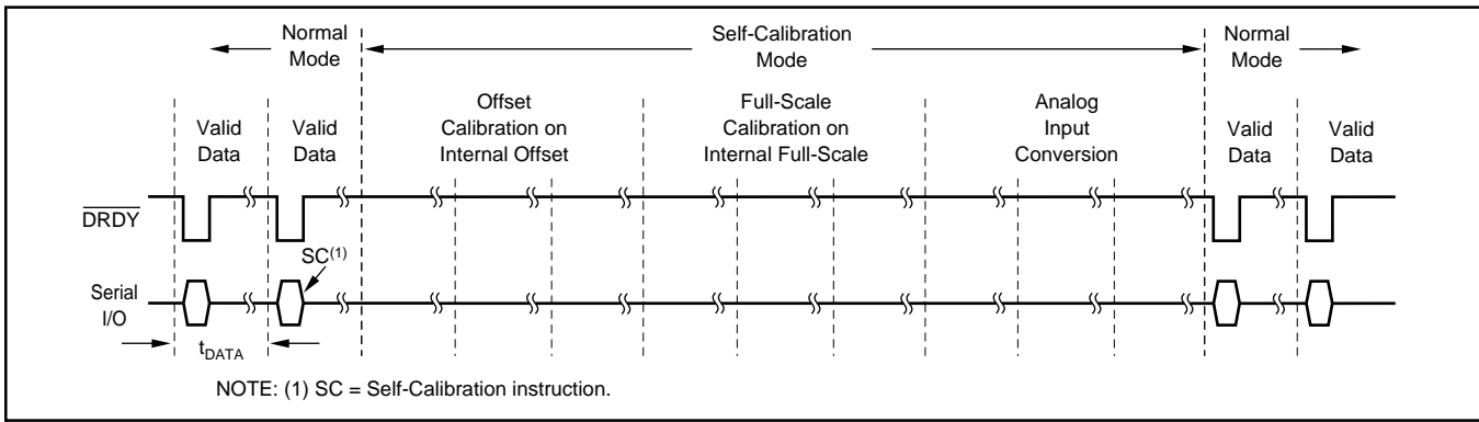
FIGURE 5. Self-Calibrating Timing Diagram.
