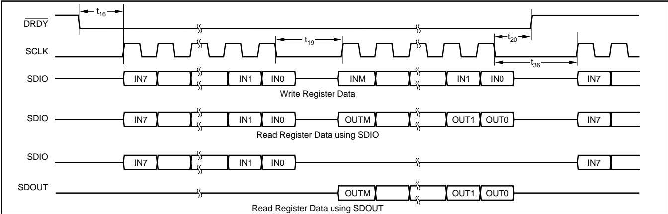
FIGURE 17. Serial Interface Timing ( \overline{CS} Tied LOW), Slave Mode.
