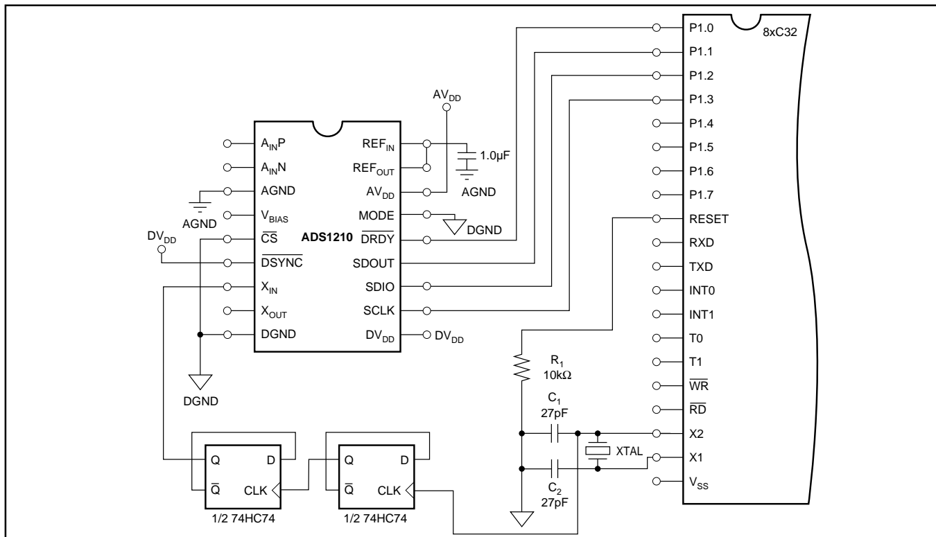
FIGURE 30. Four-Wire Interface with a 8xC32 Microprocessor.
