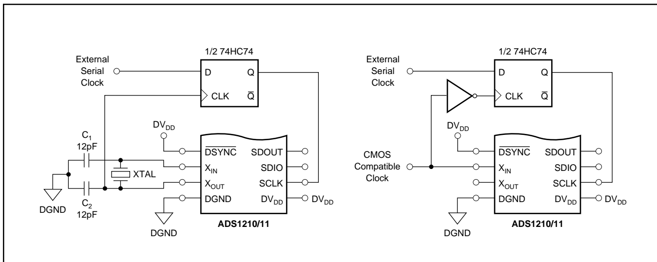
FIGURE 27. Circuits to Synchronize an External Serial Clock to the X_{IN} Input.
