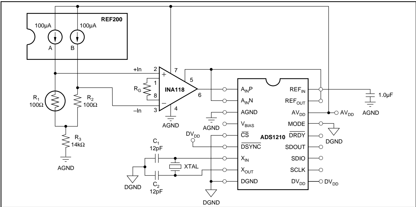
FIGURE 39. PT100 Interface.
