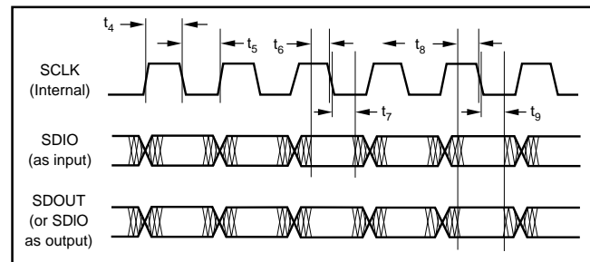
FIGURE 14. Serial Input/Output Timing, Master Mode.
