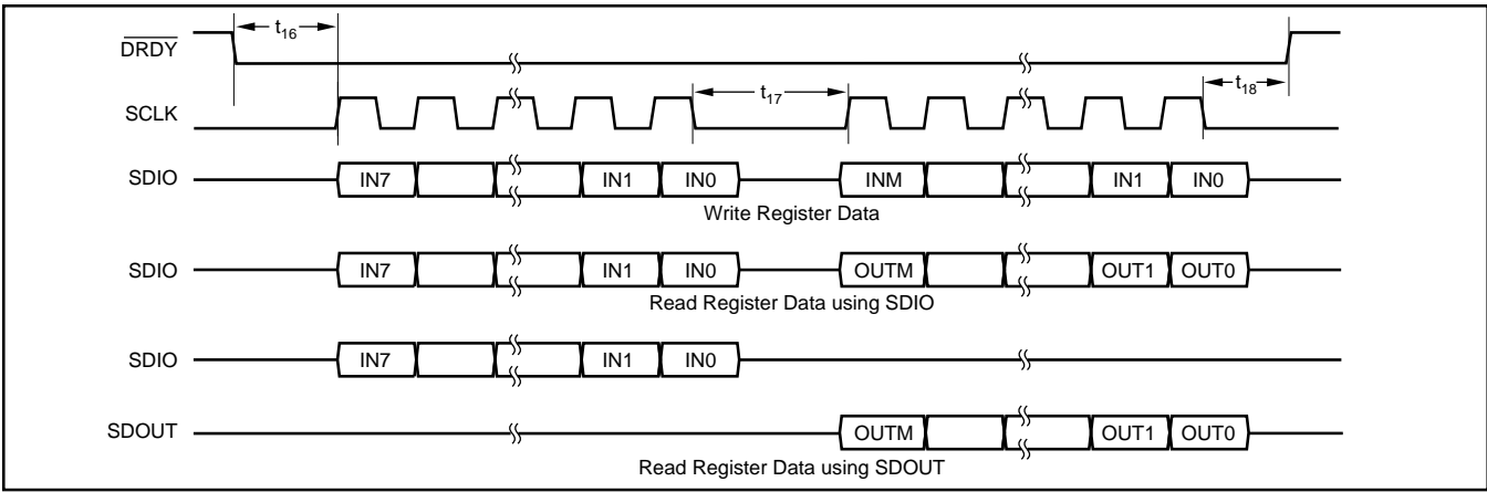
FIGURE 16. Serial Interface Timing ( \overline{CS} Tied LOW), Master Mode.
